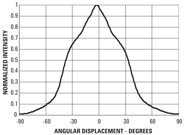
Figure 6. Representative Spatial Radiation Pattern for — major axis
